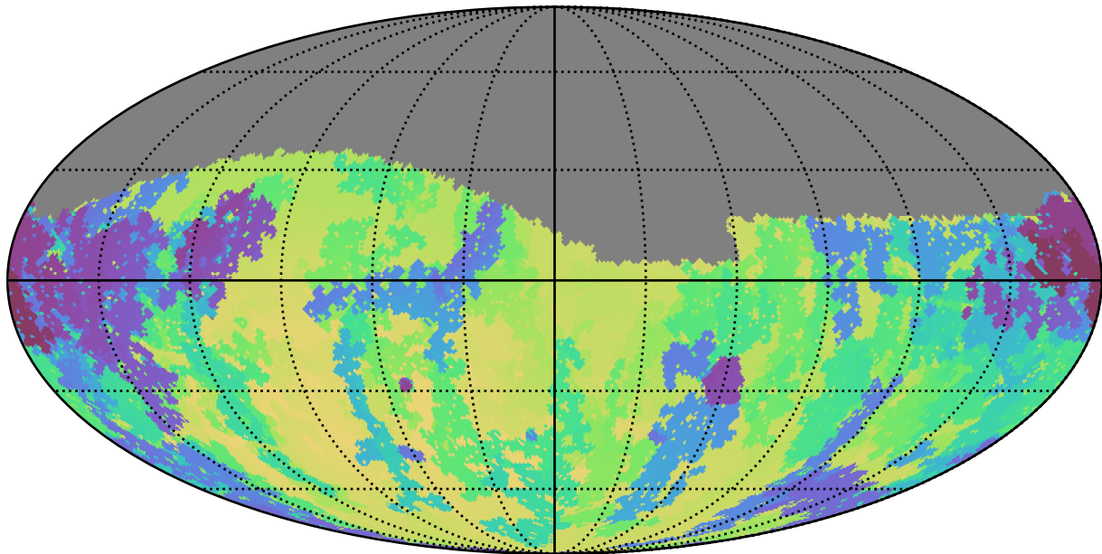
too_elab_r16_d3_giz_v3.4_10yrs Yr 1 g band: Min skyBrightness
