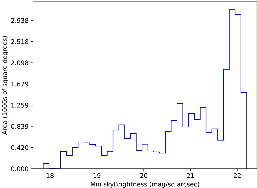
too_elab_r16_d3_giz_v3.4_10yrs Yr 1 g band: Min skyBrightness
