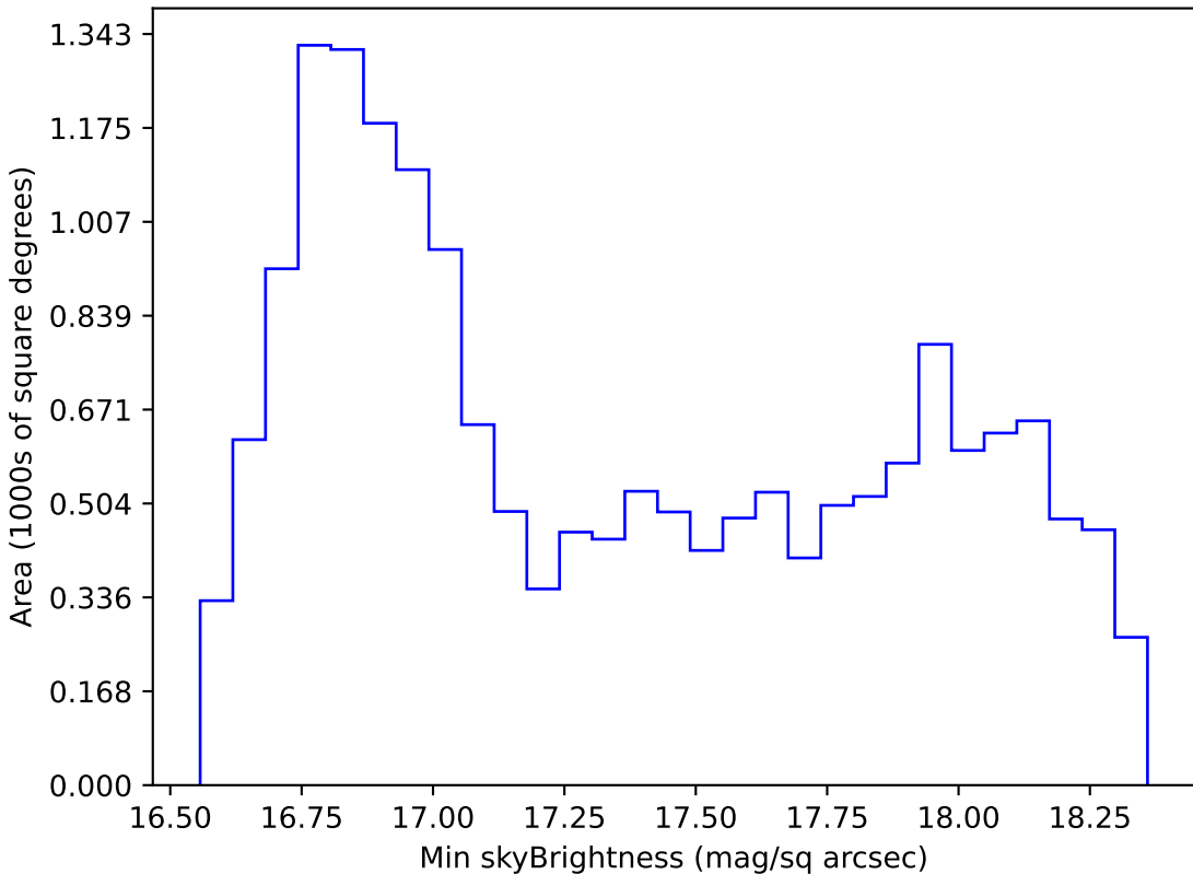
too_elab_r16_d3_giz_v3.4_10yrs WFD z band: Min skyBrightness
