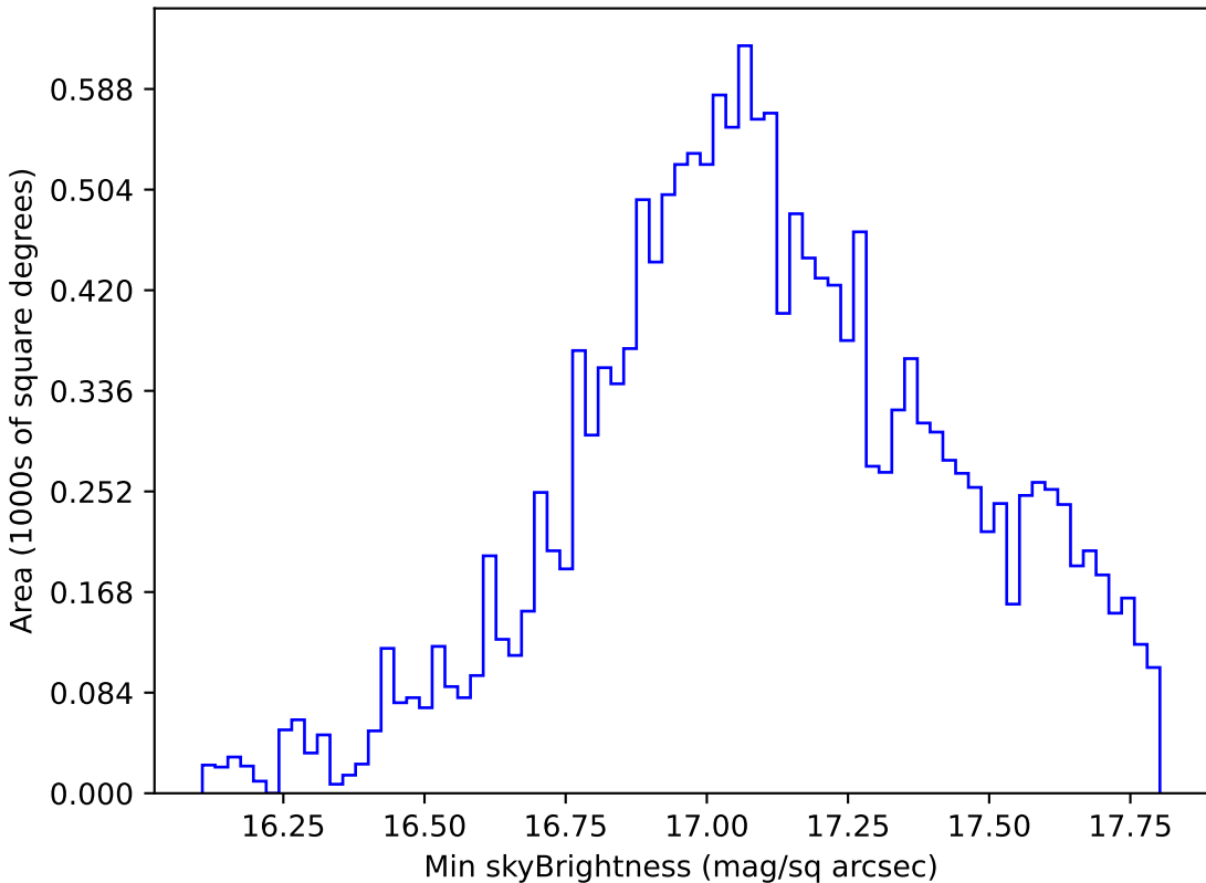
too_elab_r16_d3_giz_v3.4_10yrs WFD y band: Min skyBrightness
