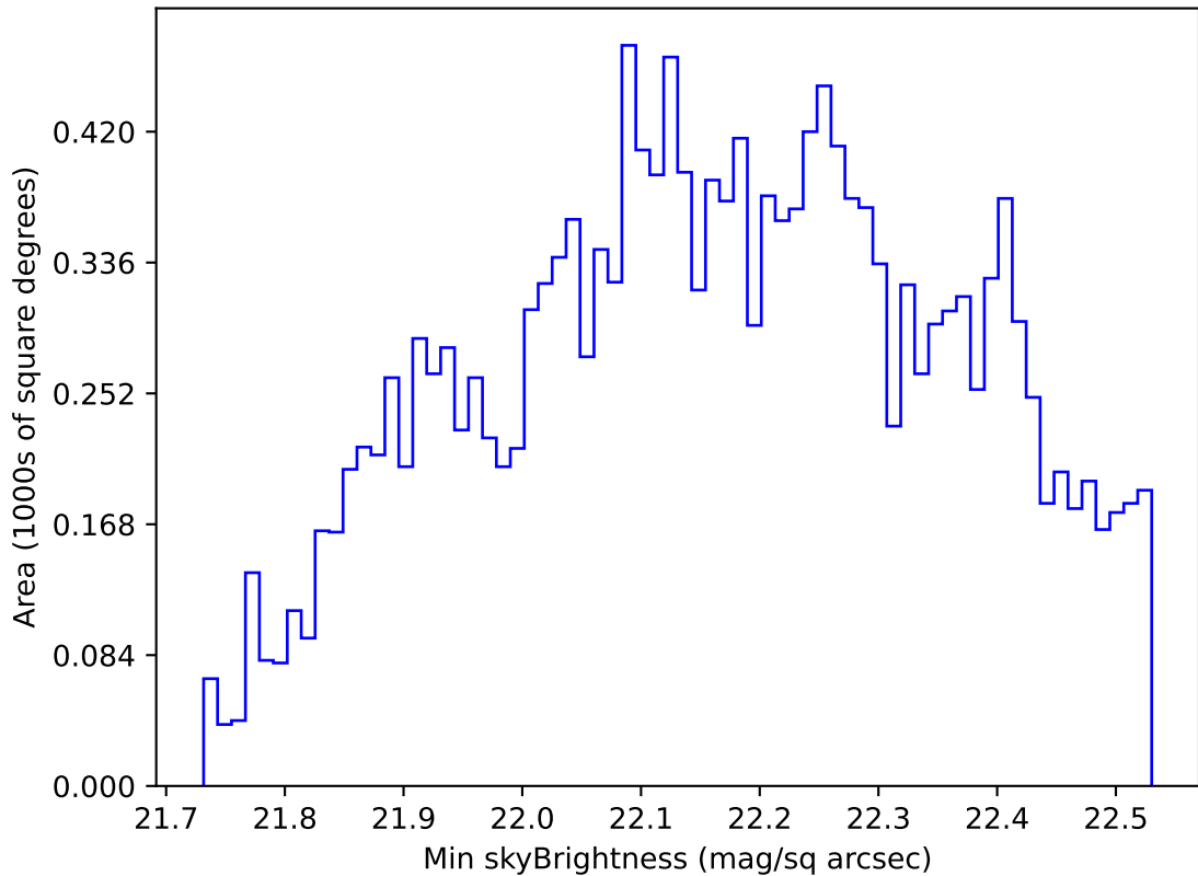
too_elab_r16_d3_giz_v3.4_10yrs WFD u band: Min skyBrightness
