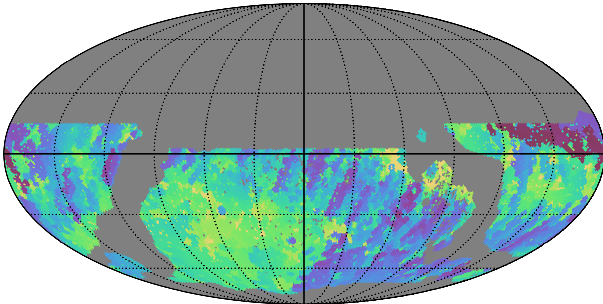
too_elab_r16_d3_giz_v3.4_10yrs WFD r band: Min skyBrightness
