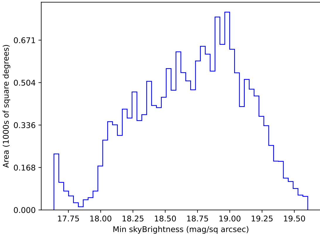
too_elab_r16_d3_giz_v3.4_10yrs WFD r band: Min skyBrightness
