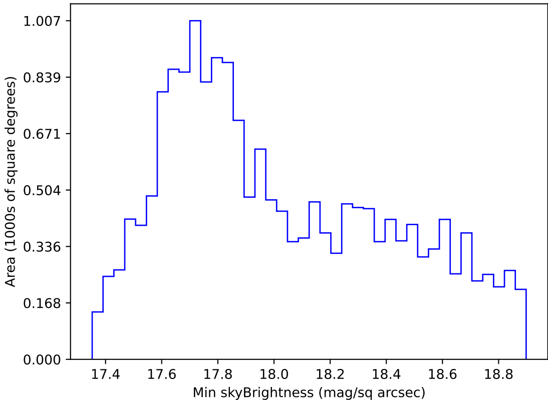
too_elab_r16_d3_giz_v3.4_10yrs WFD i band: Min skyBrightness
