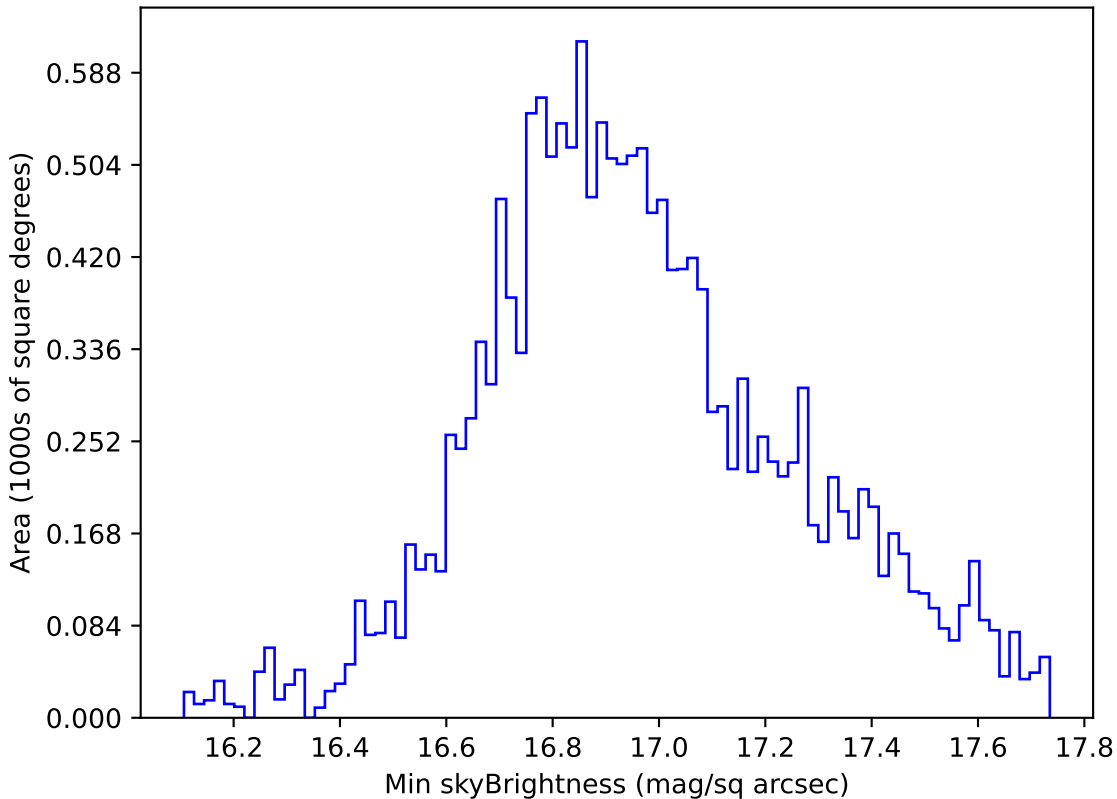
too_elab_r16_d3_giz_v3.4_10yrs WFD all bands: Min skyBrightness
