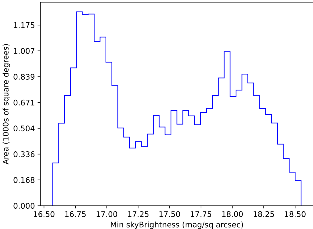
too_elab_r16_d3_giz_v3.4_10yrs All sky z band: Min skyBrightness
