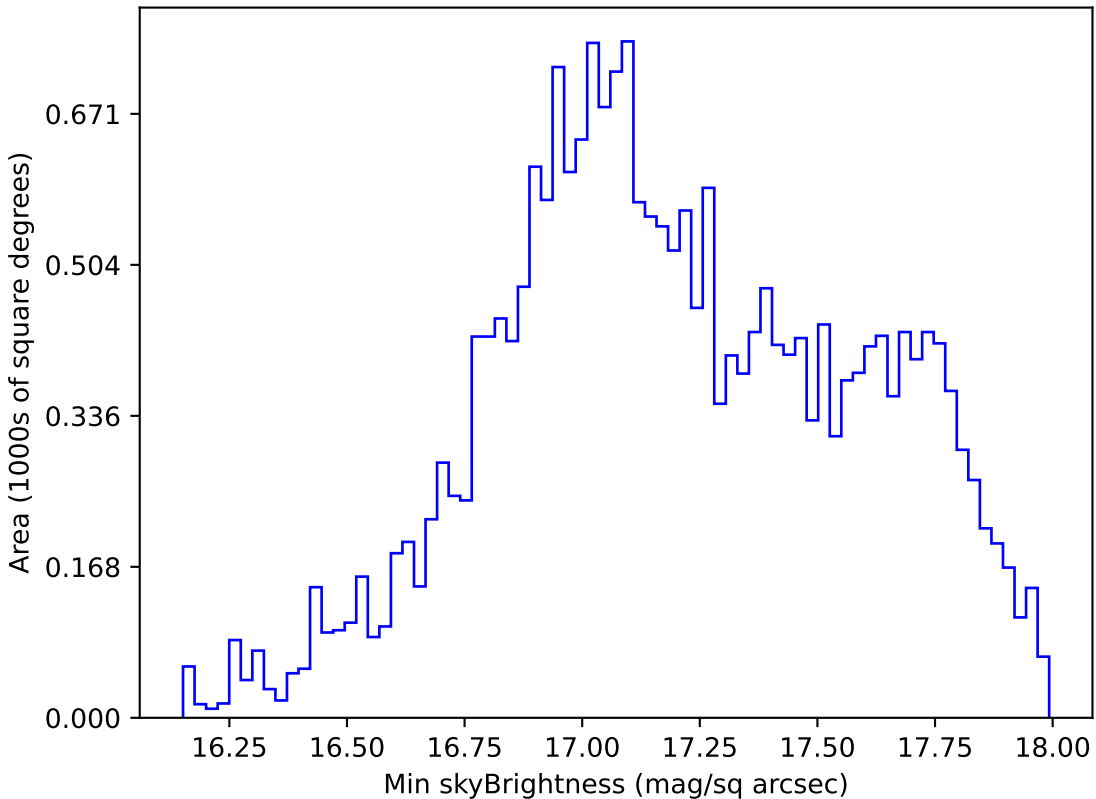
too_elab_r16_d3_giz_v3.4_10yrs All sky y band: Min skyBrightness
