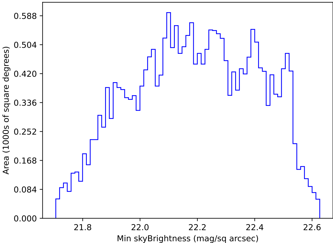
too_elab_r16_d3_giz_v3.4_10yrs All sky u band: Min skyBrightness
