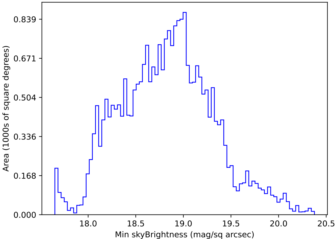
too_elab_r16_d3_giz_v3.4_10yrs All sky r band: Min skyBrightness
