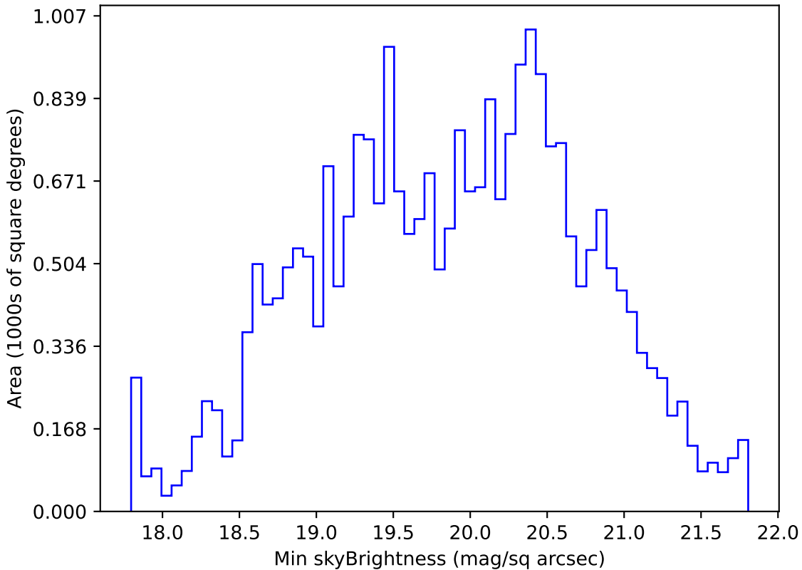
too_elab_r16_d3_giz_v3.4_10yrs All sky g band: Min skyBrightness
