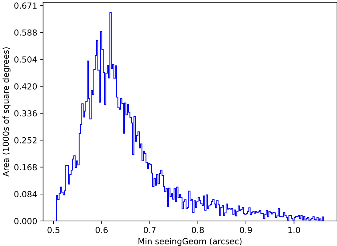
too_elab_r16_d3_giz_v3.4_10yrs Yr 1 z band: Min seeingGeom
