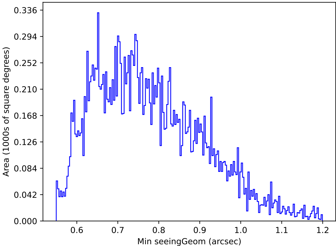
too_elab_r16_d3_giz_v3.4_10yrs Yr 1 u band: Min seeingGeom
