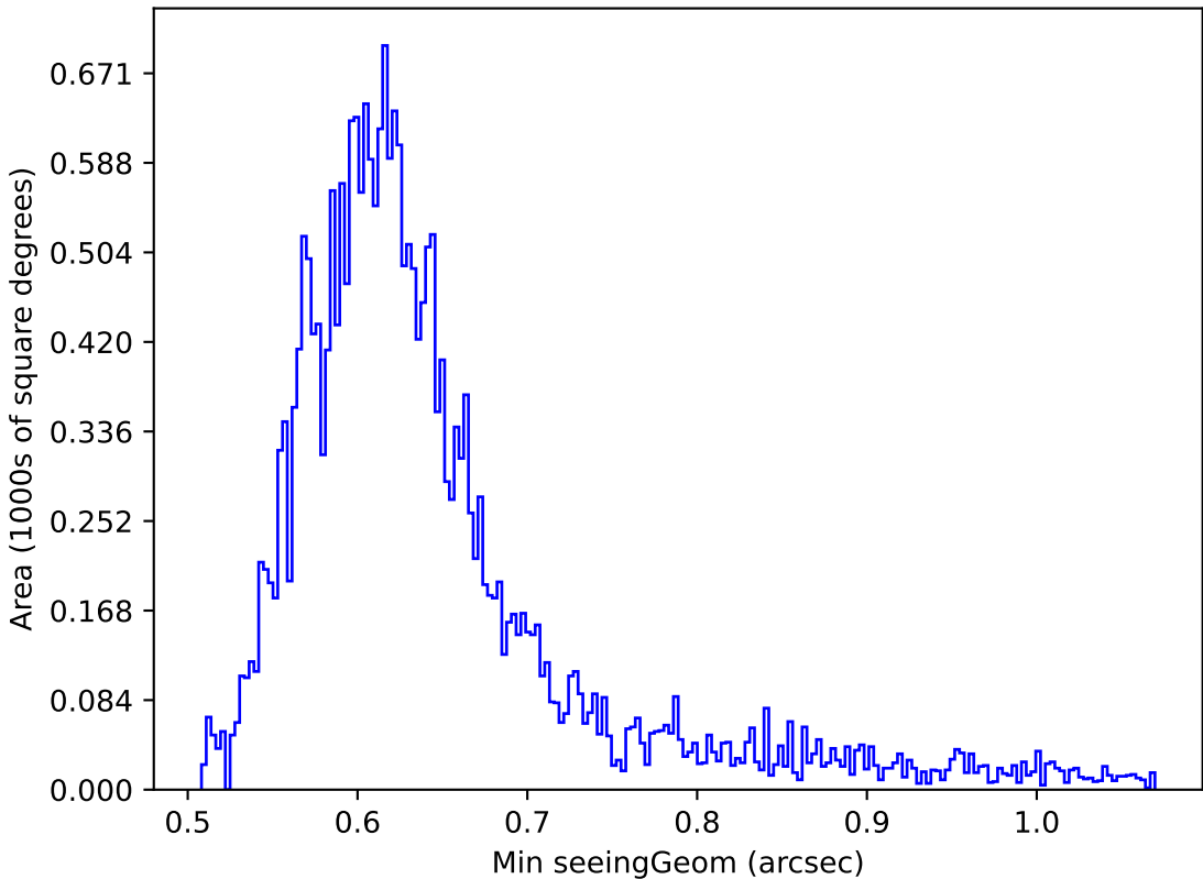
too_elab_r16_d3_giz_v3.4_10yrs Yr 1 r band: Min seeingGeom
