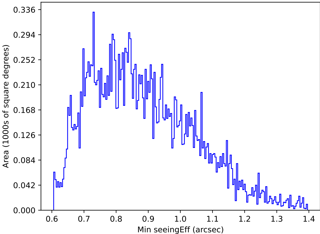
too_elab_r16_d3_giz_v3.4_10yrs Yr 1 u band: Min seeingEff
