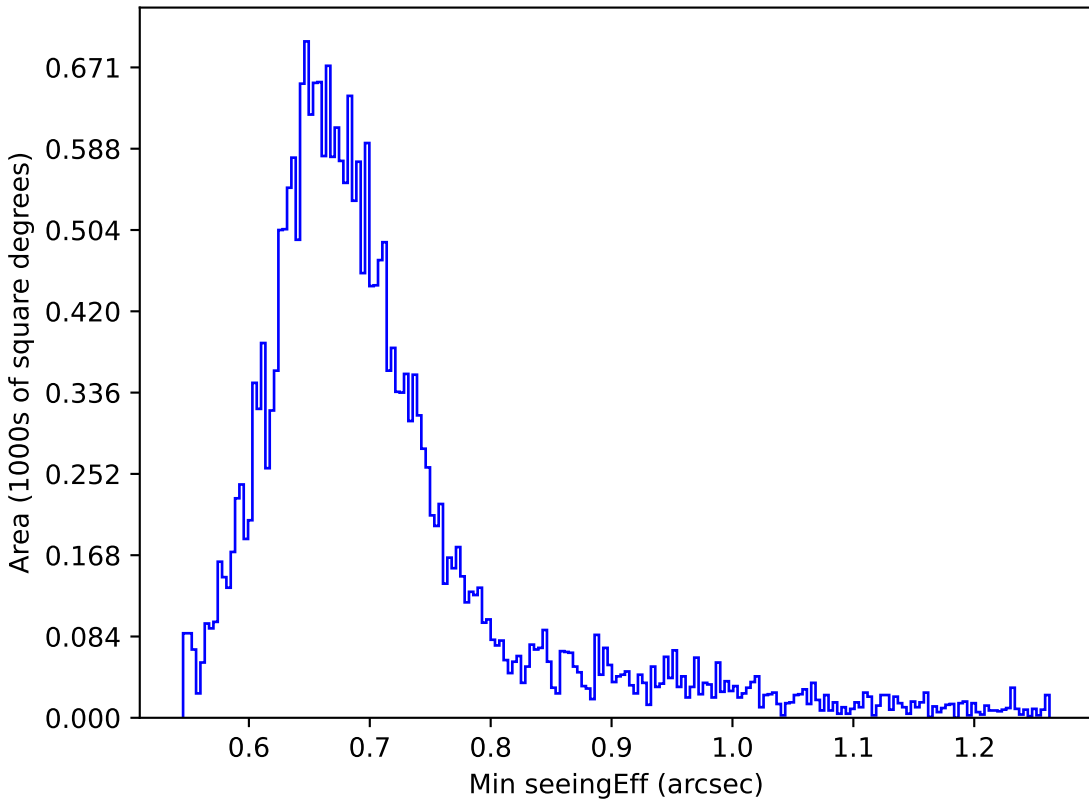
too_elab_r16_d3_giz_v3.4_10yrs Yr 1 i band: Min seeingEff
