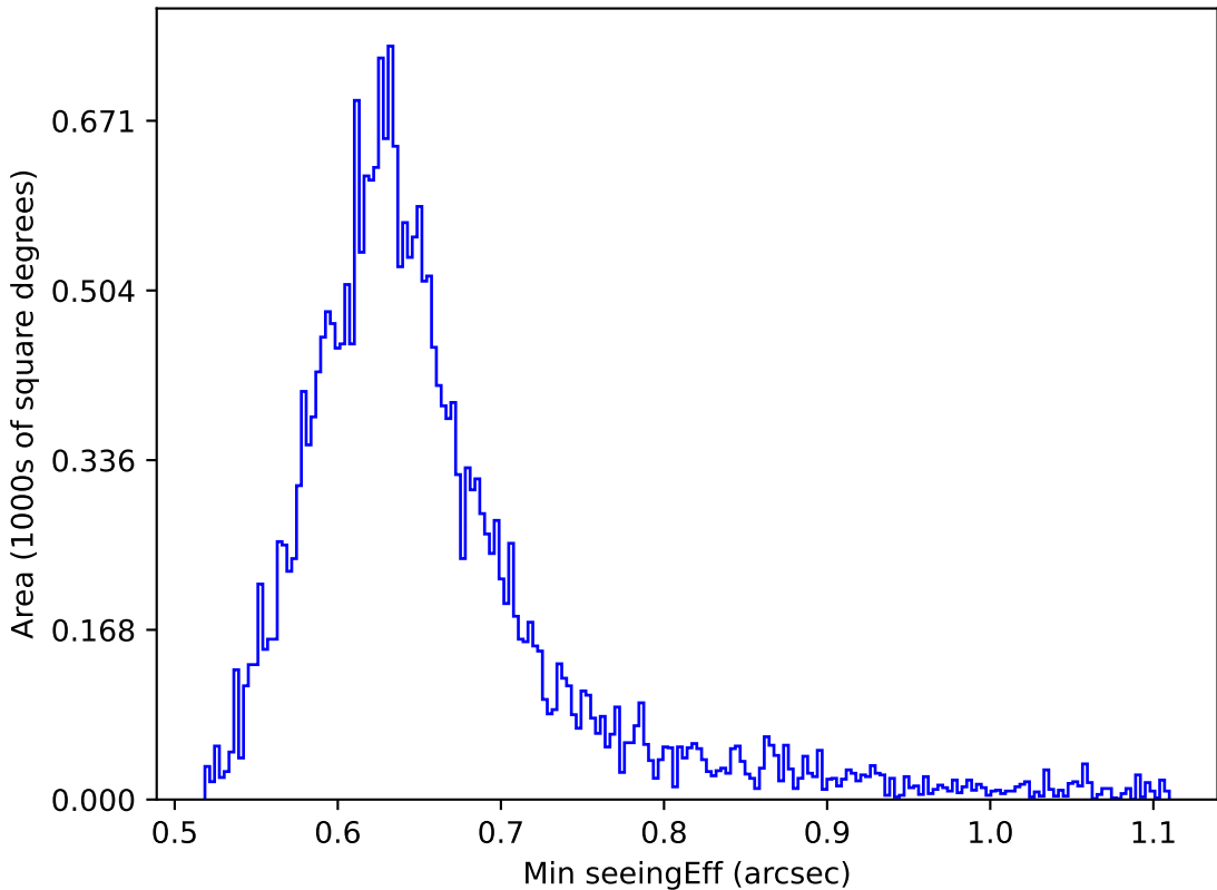
too_elab_r16_d3_giz_v3.4_10yrs Yr 1 all bands: Min seeingEff
