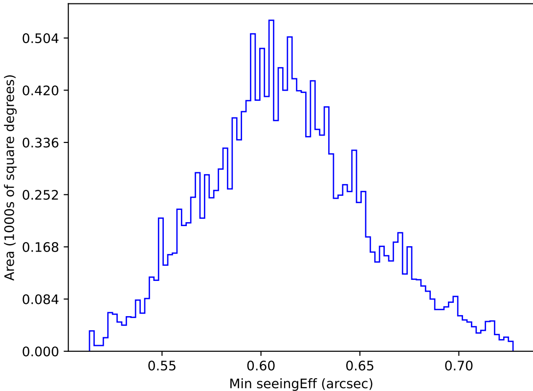
too_elab_r16_d3_giz_v3.4_10yrs WFD z band: Min seeingEff
