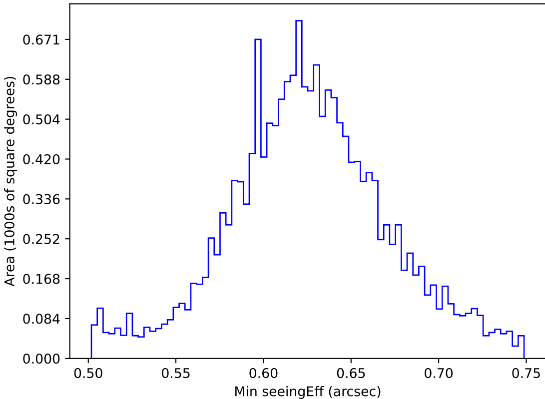
too_elab_r16_d3_giz_v3.4_10yrs WFD y band: Min seeingEff
