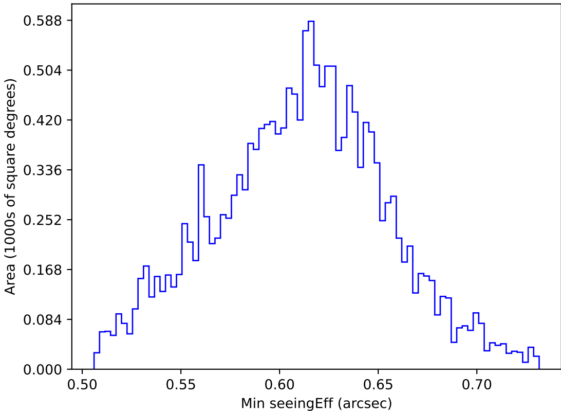
too_elab_r16_d3_giz_v3.4_10yrs WFD r band: Min seeingEff
