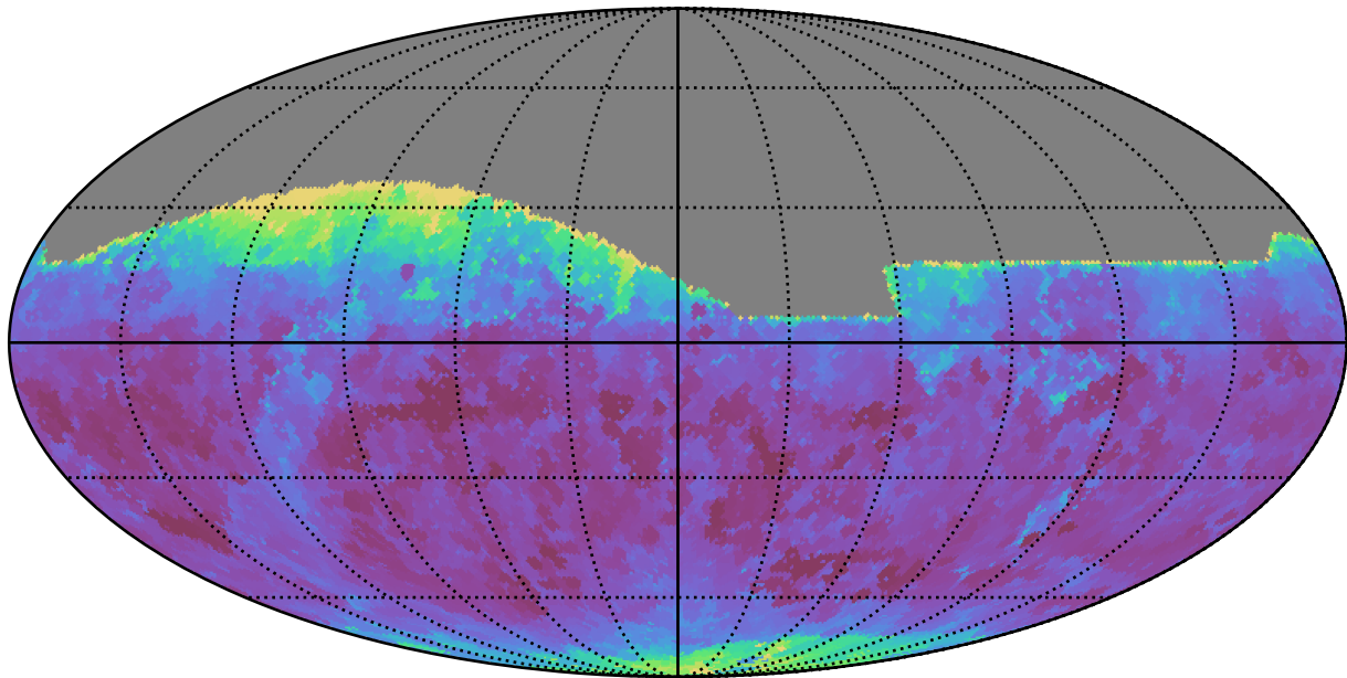
too_elab_r16_d3_giz_v3.4_10yrs All sky z band: Min seeingEff
