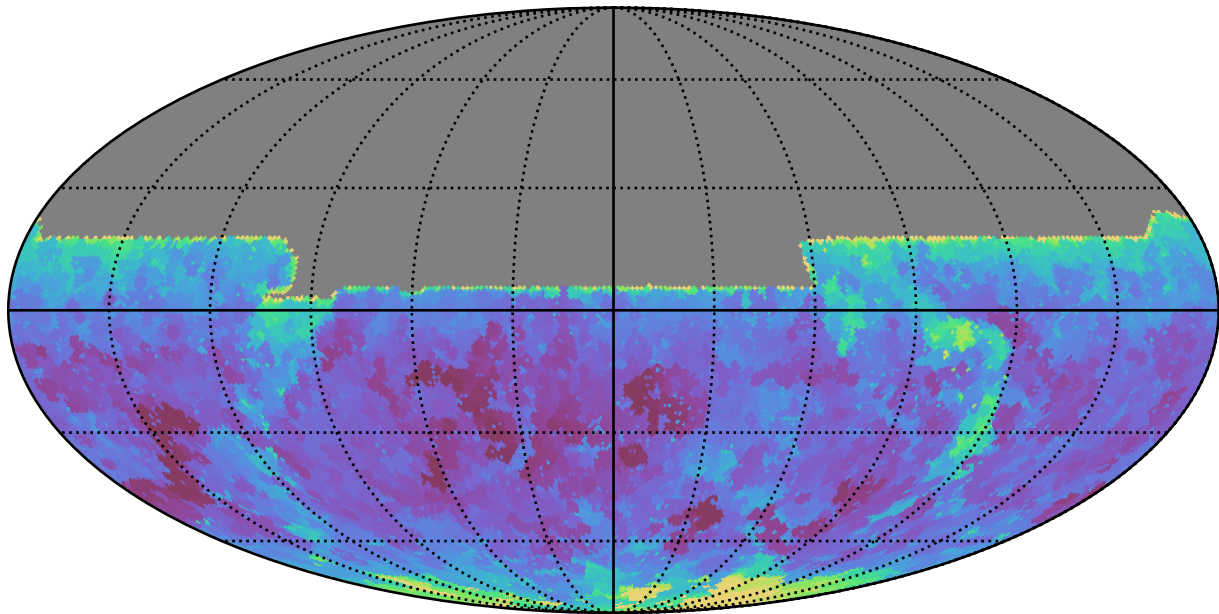
too_elab_r16_d3_giz_v3.4_10yrs All sky y band: Min seeingEff
