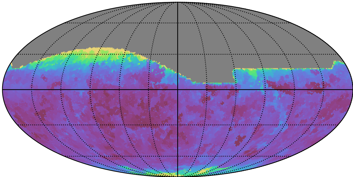
too_elab_r16_d3_giz_v3.4_10yrs All sky r band: Min seeingEff
