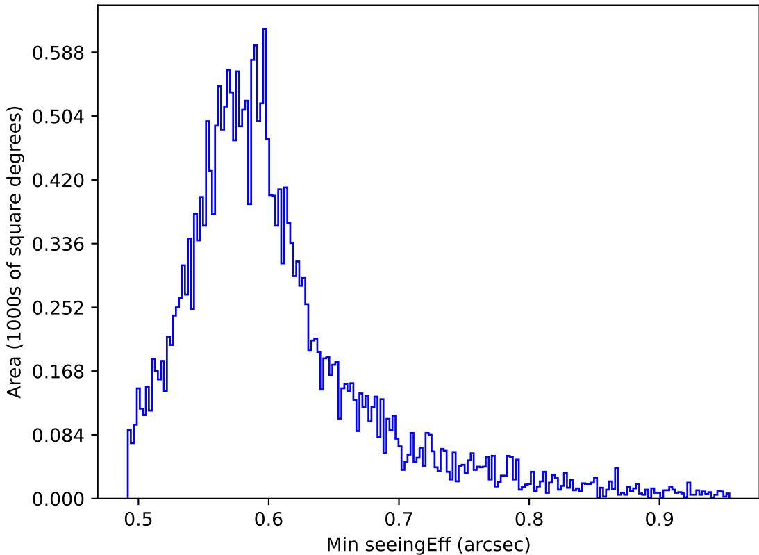
too_elab_r16_d3_giz_v3.4_10yrs All sky all bands: Min seeingEff
