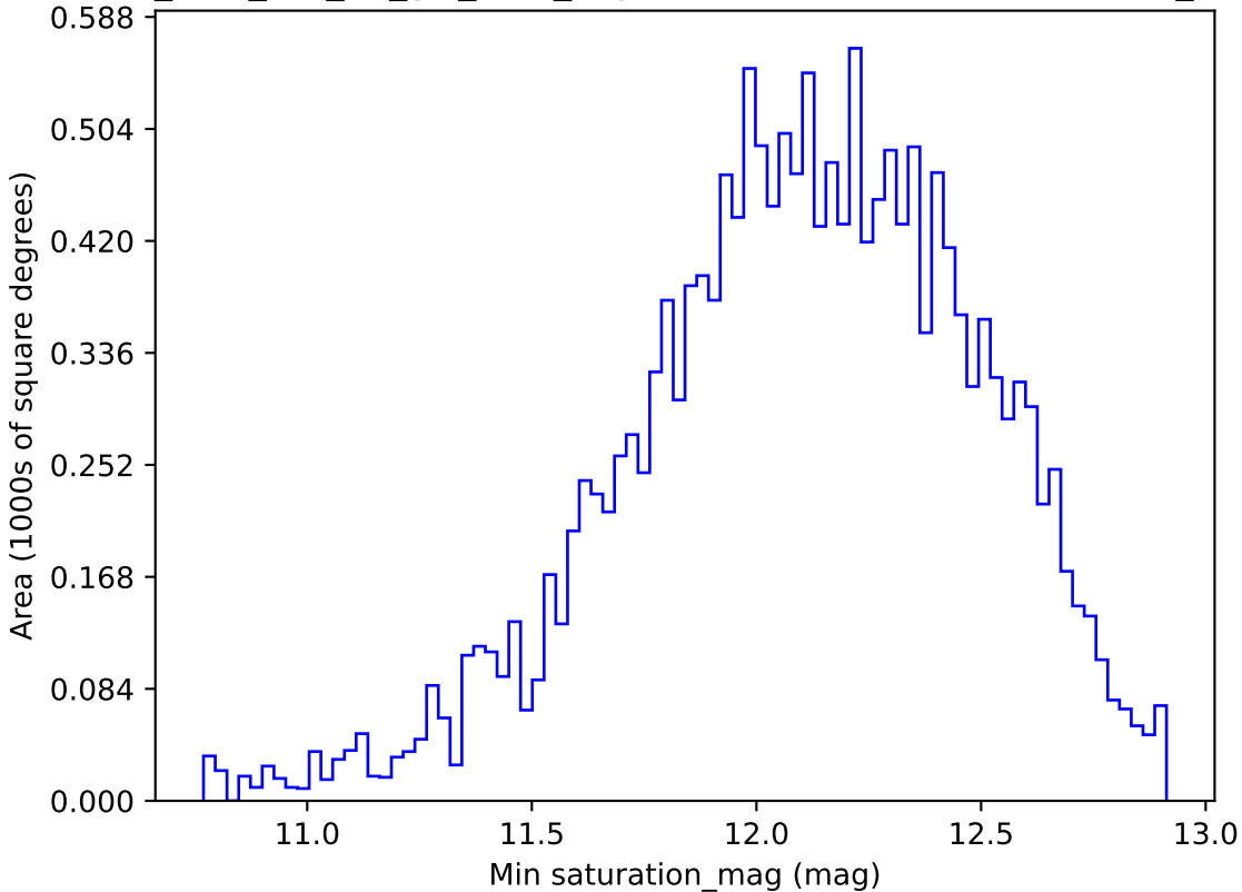
too_elab_r16_d3_giz_v3.4_10yrs WFD z band: Min saturation_mag
