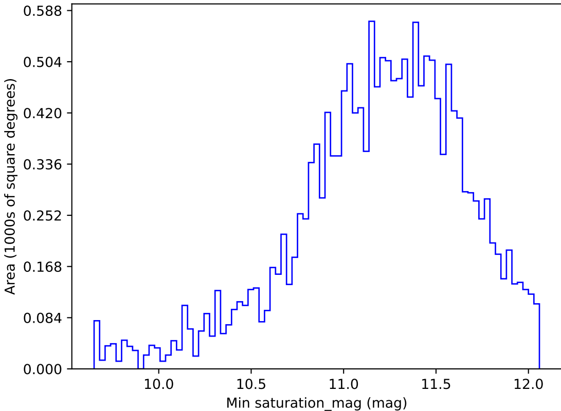
too_elab_r16_d3_giz_v3.4_10yrs WFD y band: Min saturation_mag
