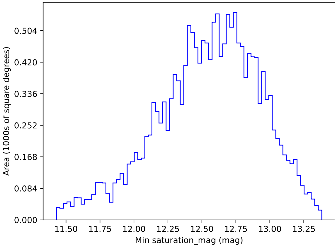
too_elab_r16_d3_giz_v3.4_10yrs WFD r band: Min saturation_mag
