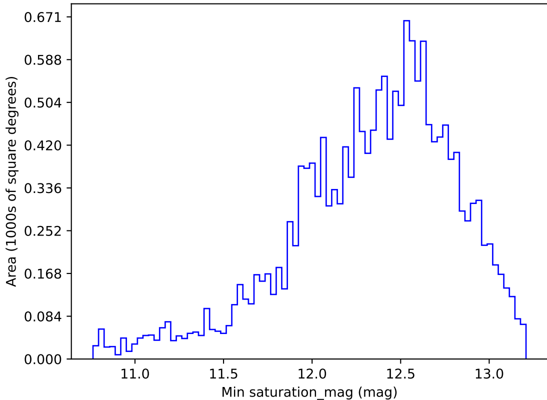
too_elab_r16_d3_giz_v3.4_10yrs WFD i band: Min saturation_mag
