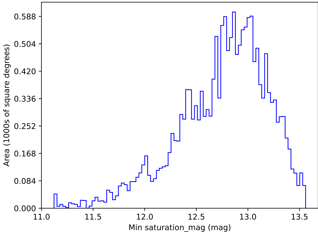
too_elab_r16_d3_giz_v3.4_10yrs WFD g band: Min saturation_mag
