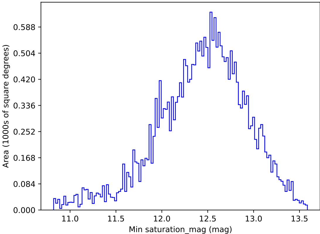
too_elab_r16_d3_giz_v3.4_10yrs All sky i band: Min saturation_mag
