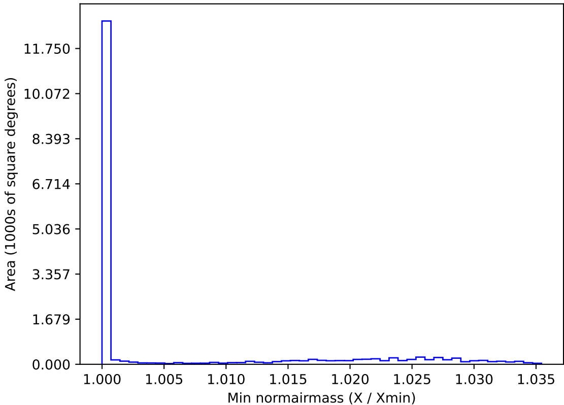
too_elab_r16_d3_giz_v3.4_10yrs WFD r band: Min normairmass
