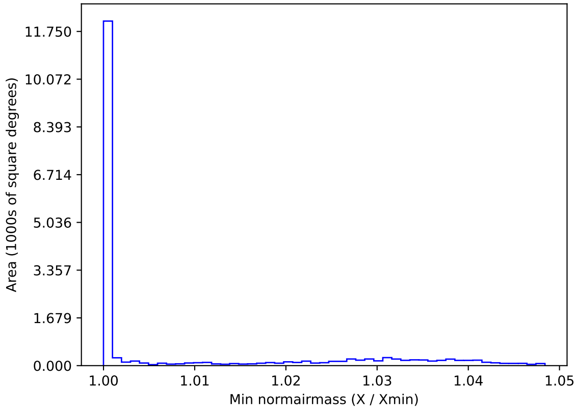
too_elab_r16_d3_giz_v3.4_10yrs WFD g band: Min normairmass
