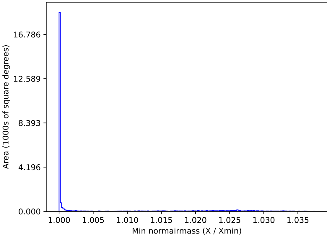
too_elab_r16_d3_giz_v3.4_10yrs All sky i band: Min normairmass
