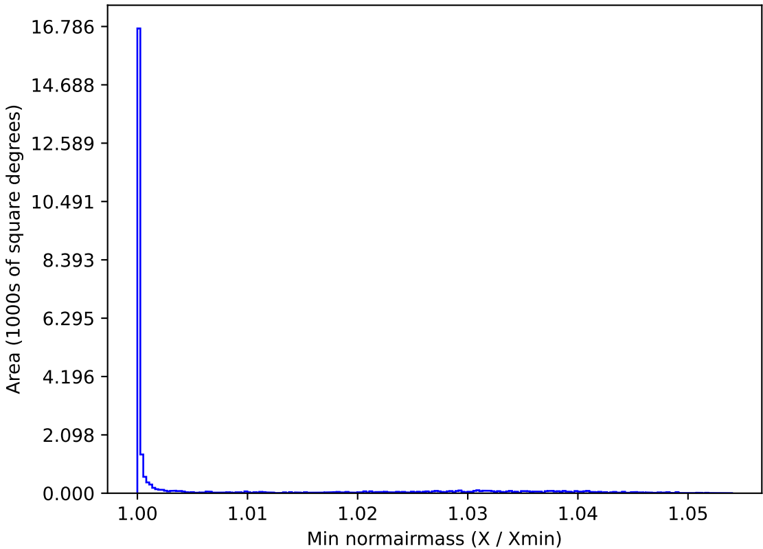
too_elab_r16_d3_giz_v3.4_10yrs All sky g band: Min normairmass
