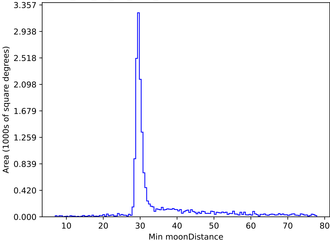
too_elab_r16_d3_giz_v3.4_10yrs WFD z band: Min moonDistance
