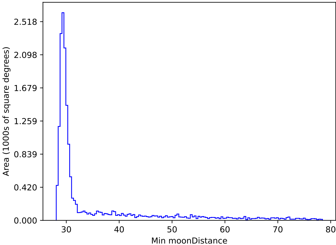
too_elab_r16_d3_giz_v3.4_10yrs WFD y band: Min moonDistance
