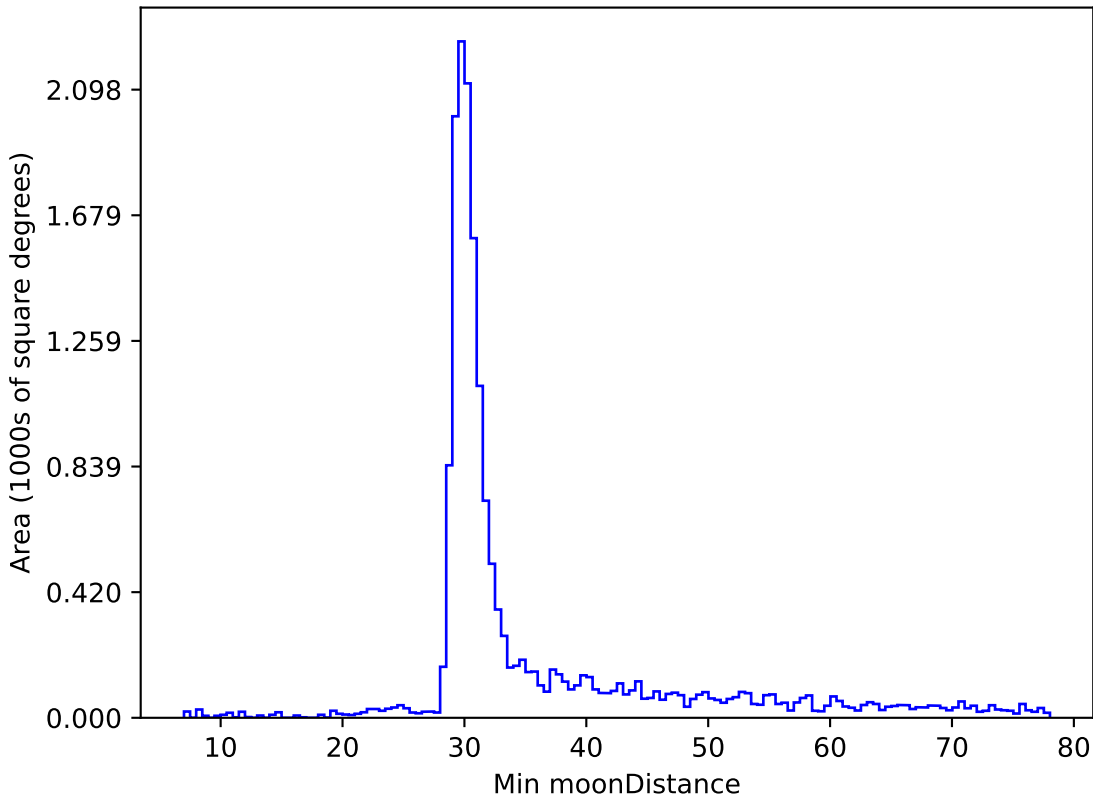
too_elab_r16_d3_giz_v3.4_10yrs WFD i band: Min moonDistance
