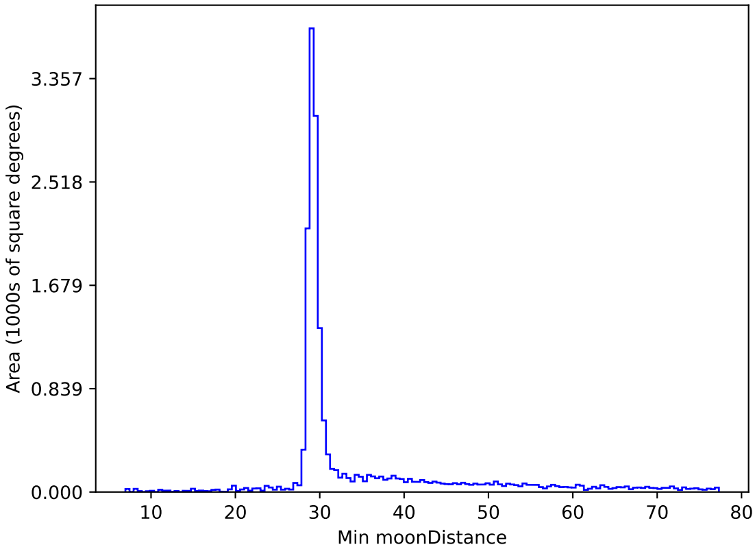
too_elab_r16_d3_giz_v3.4_10yrs WFD all bands: Min moonDistance
