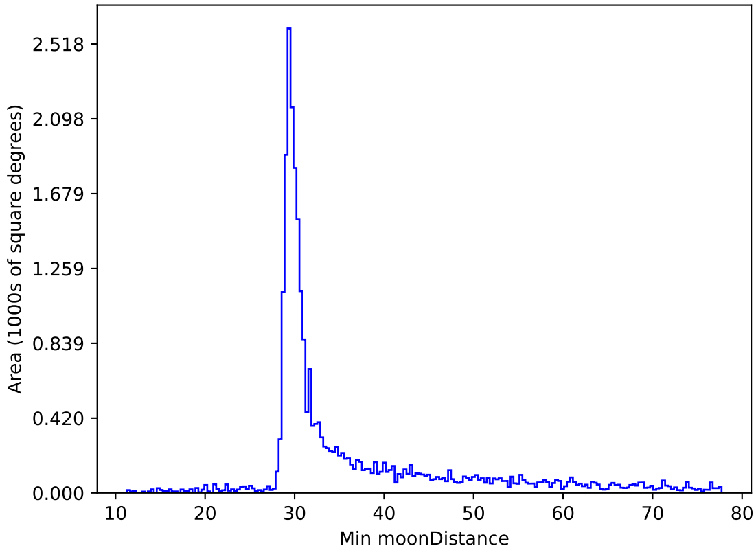
too_elab_r16_d3_giz_v3.4_10yrs All sky z band: Min moonDistance
