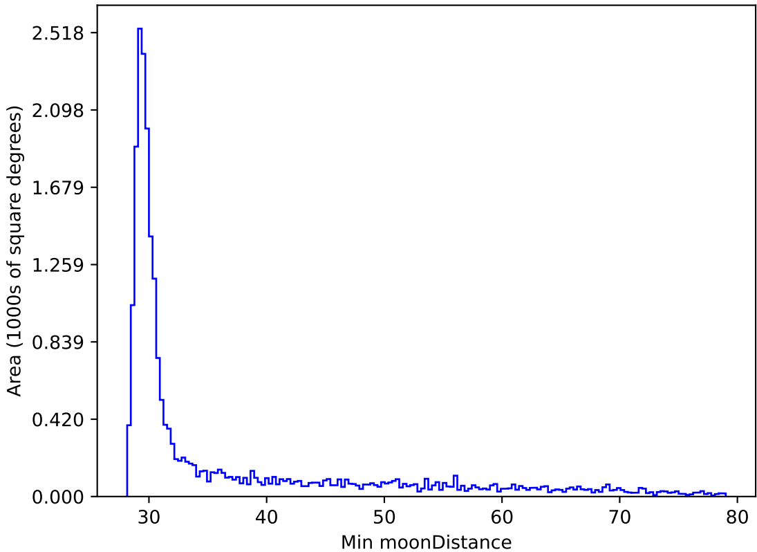
too_elab_r16_d3_giz_v3.4_10yrs All sky y band: Min moonDistance
