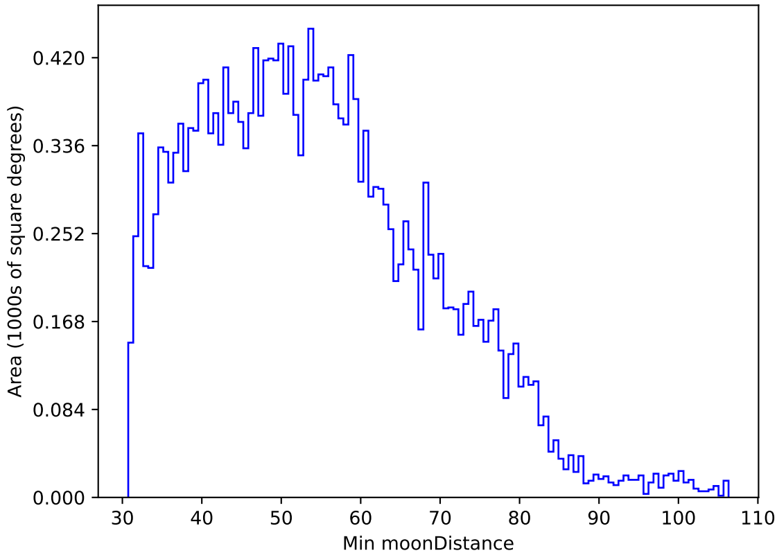
too_elab_r16_d3_giz_v3.4_10yrs All sky u band: Min moonDistance
