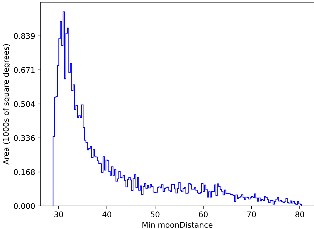
too_elab_r16_d3_giz_v3.4_10yrs All sky r band: Min moonDistance
