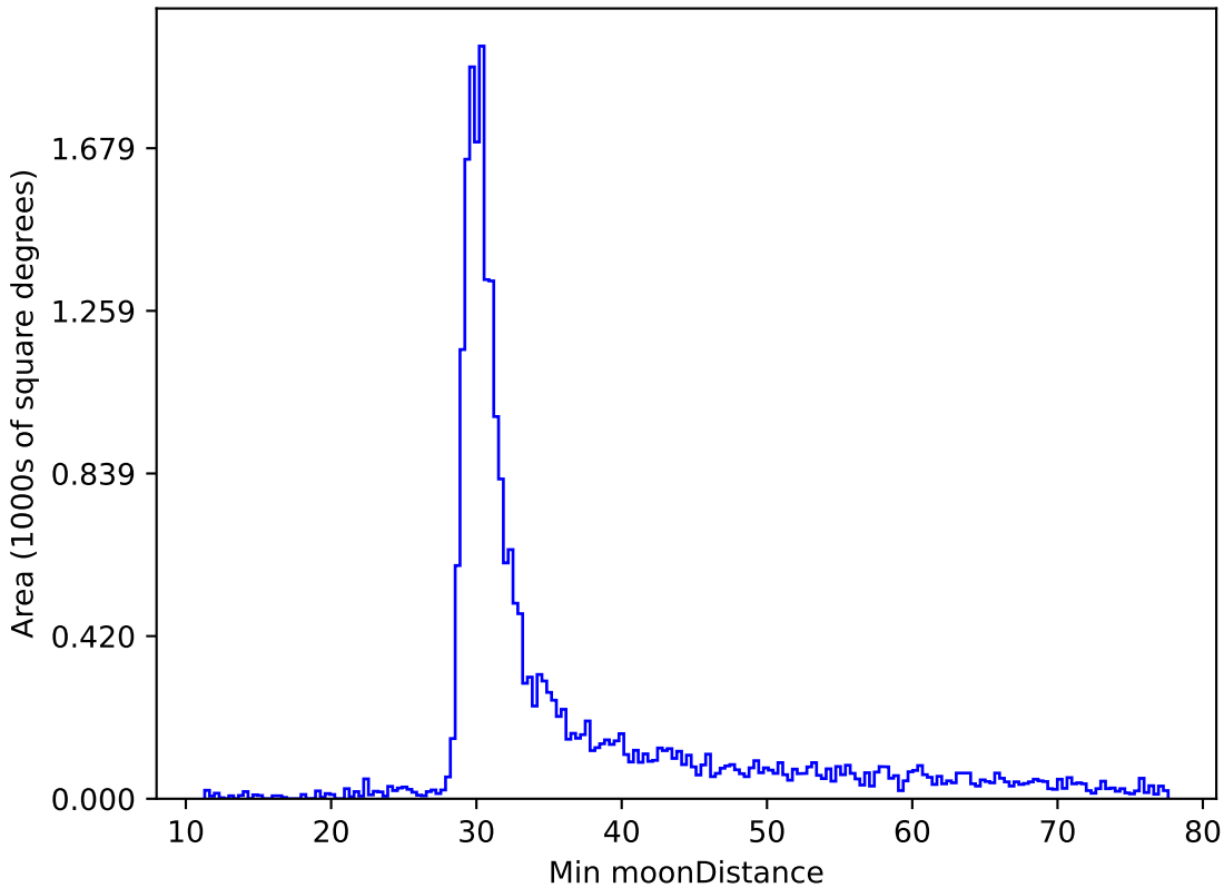
too_elab_r16_d3_giz_v3.4_10yrs All sky i band: Min moonDistance
