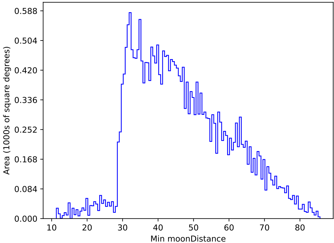
too_elab_r16_d3_giz_v3.4_10yrs All sky g band: Min moonDistance
