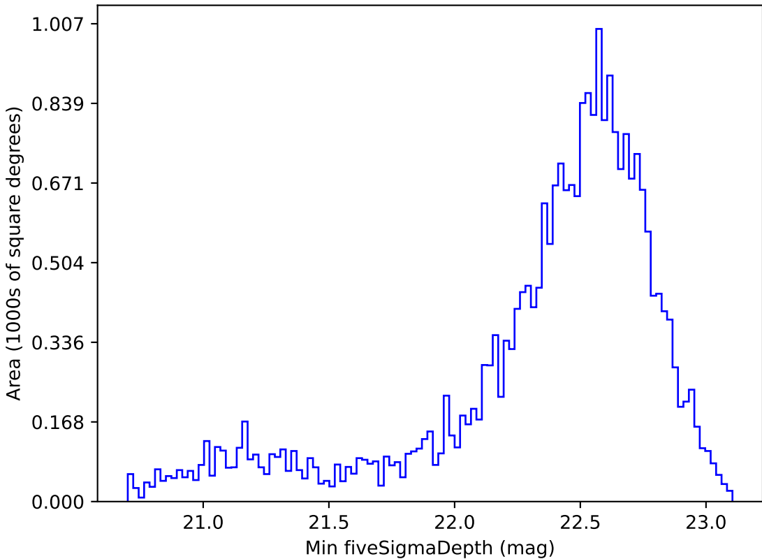
too_elab_r16_d3_giz_v3.4_10yrs Yr 1 z band: Min fiveSigmaDepth
