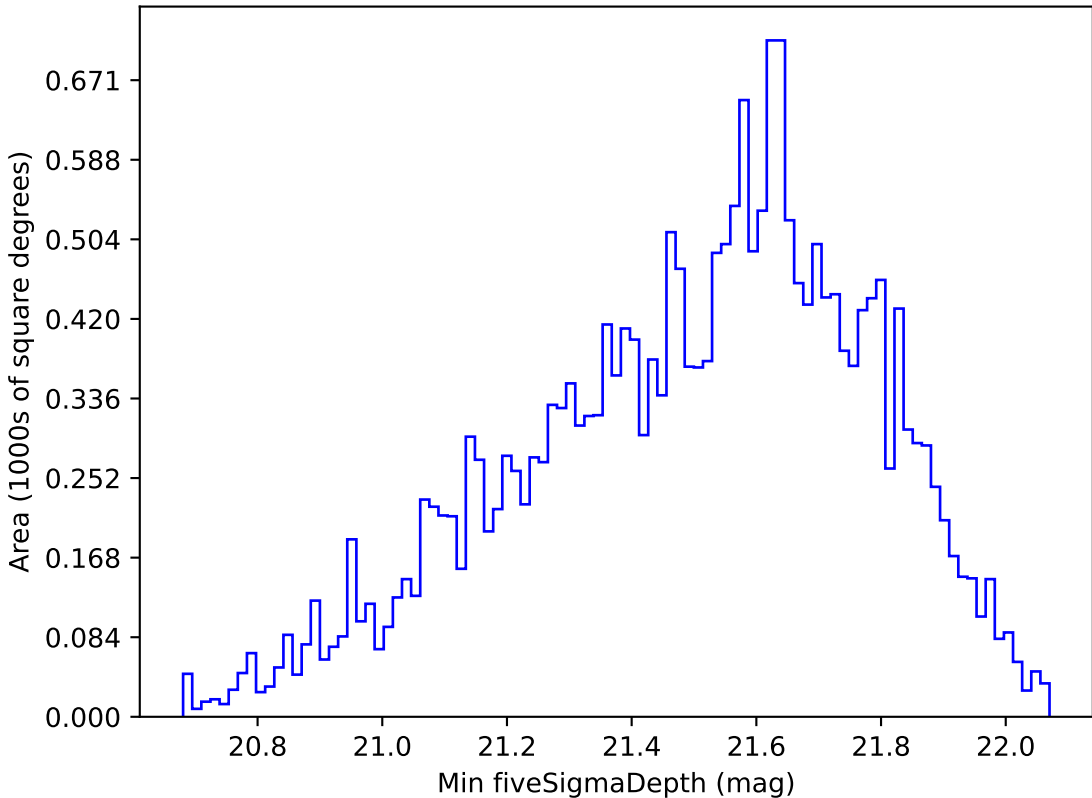
too_elab_r16_d3_giz_v3.4_10yrs Yr 1 y band: Min fiveSigmaDepth
