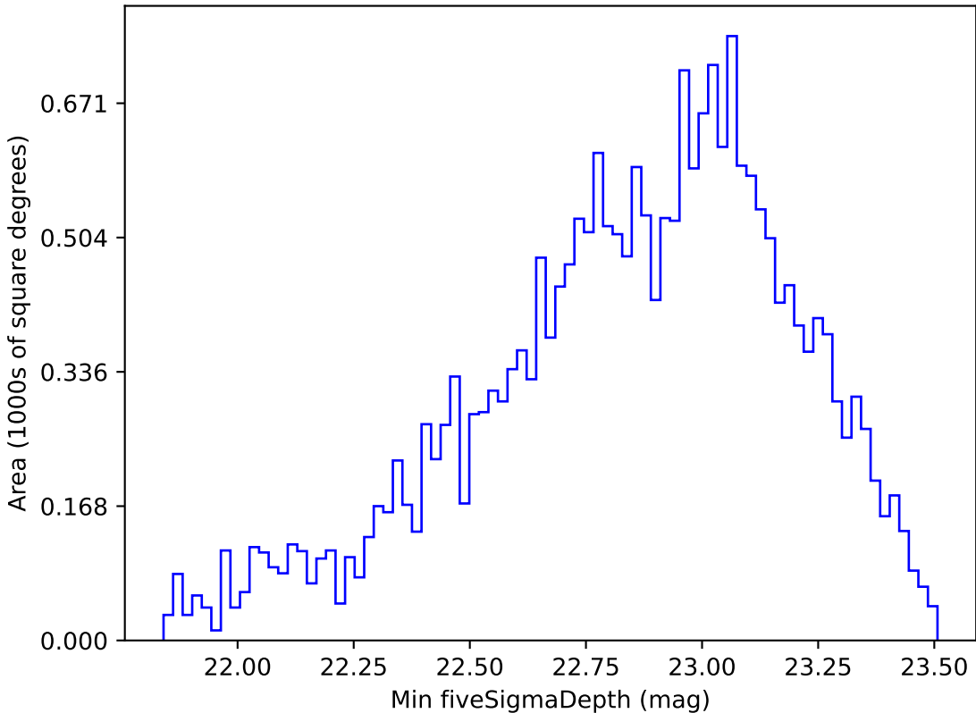
too_elab_r16_d3_giz_v3.4_10yrs Yr 1 u band: Min fiveSigmaDepth
